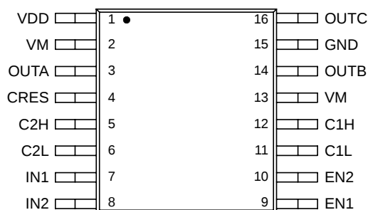
Figure 3. 17517 Pin Connections
