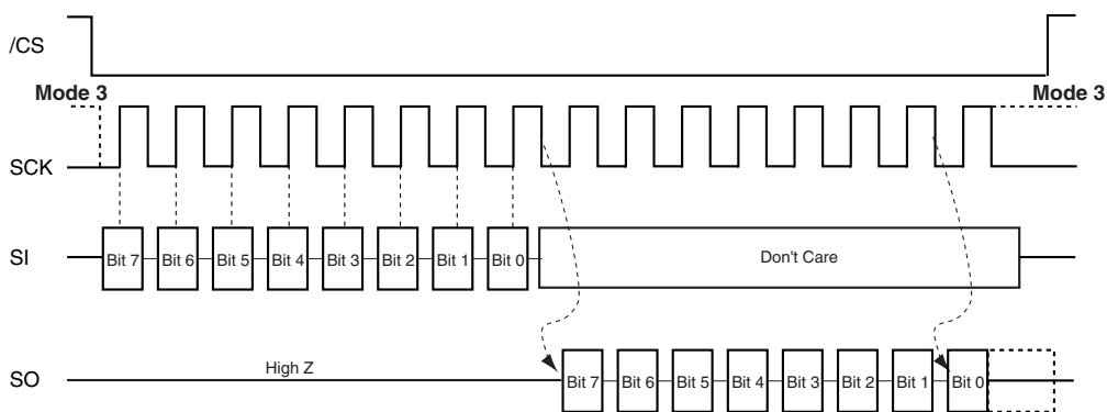
FIGURE 2. SPI Protocol
