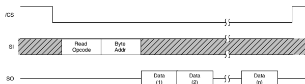
FIGURE 5. Read Sequence
