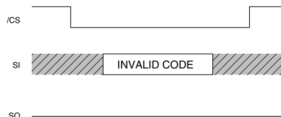
FIGURE 14. Invalid Op-Code
