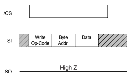
FIGURE 9. Byte Write
