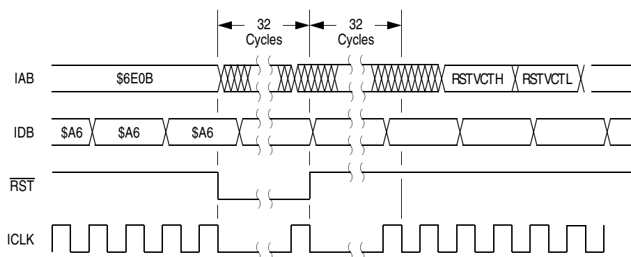
Figure 4-17. Wait Recovery from Internal Reset
