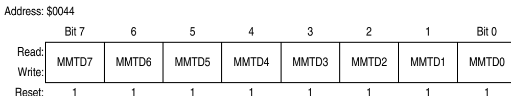
Figure 8-8. Multi-Master IIC Data Transmit Register (MMDTR)
