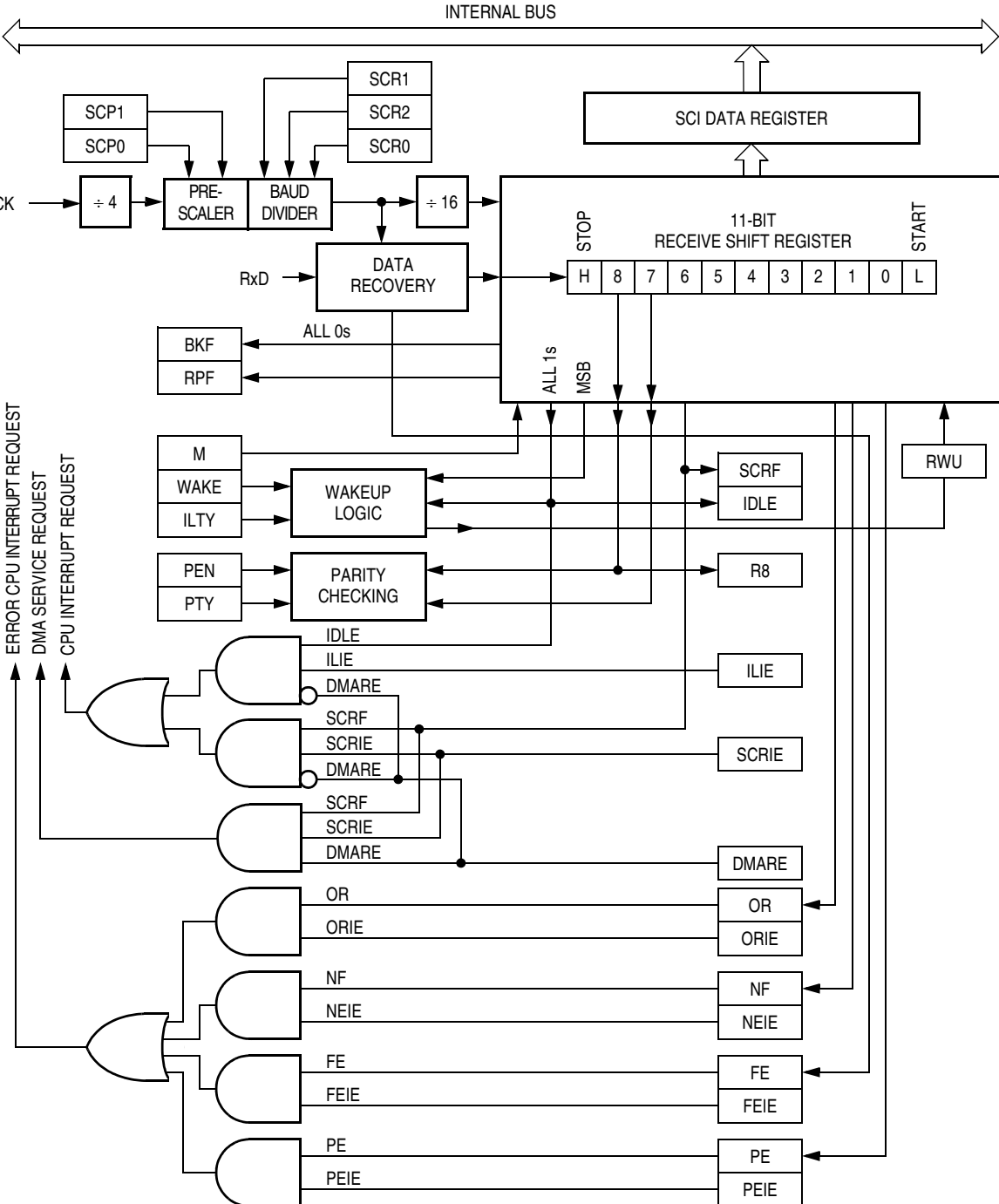
Figure 7-5. SCI Receiver Block Diagram
