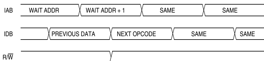
Figure 4-15. Wait Mode Entry Timing
