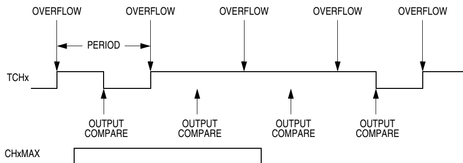
Figure 6-11. CHxMAX Latency
