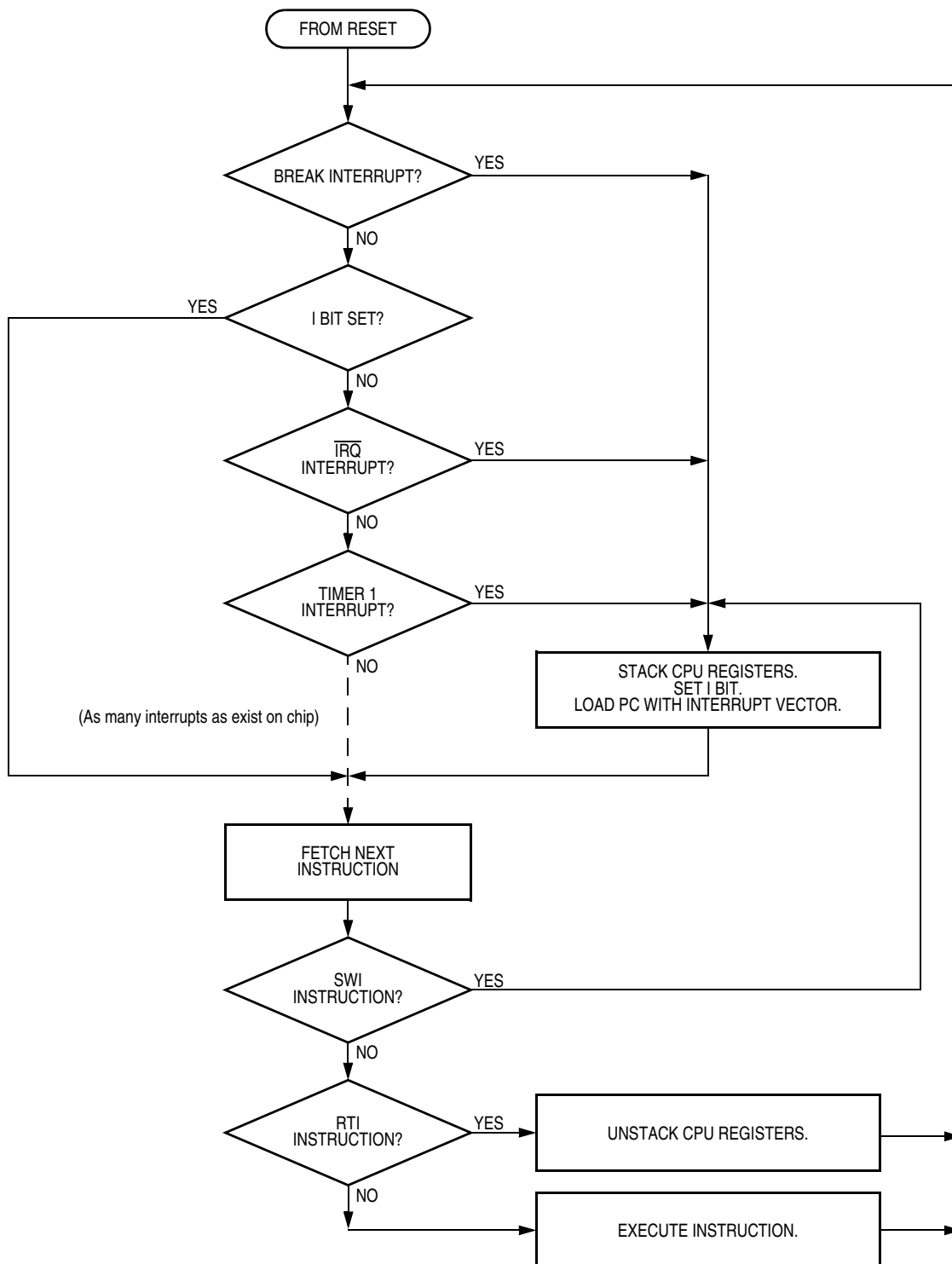
Figure 4-8. Interrupt Processing
