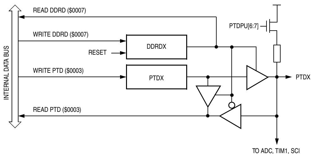
Figure 10-12. Port D I/O Circuit
