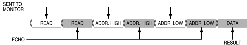
Figure 16-12. Read Transaction
