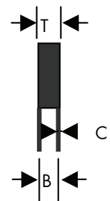
PAD LAYOUT
