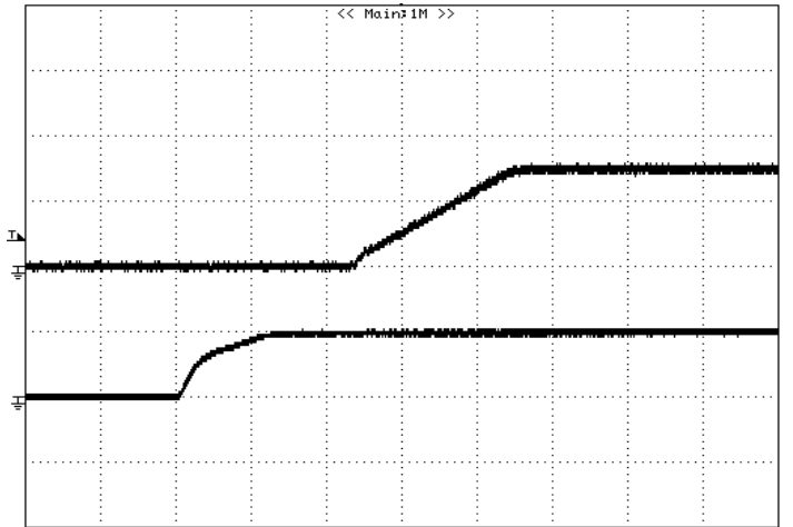
Figure 16: Turn on delay time at 5Vin, 1.5V/5A out Top: Vout, 1V/div, Bottom: 5V/div; 2mS/div
