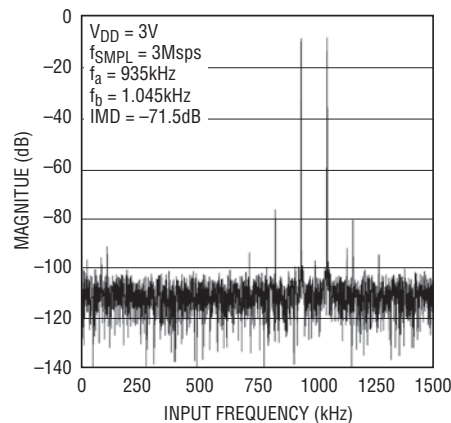
Figure 9b. LTC2366 Intermodulation Distortion Plot
