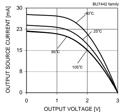
Fig.124 Output Source Current – Output Voltage (VDD=3.0[V])
