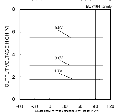
Fig.52 Output Voltage High - Ambient Temperature (RL=10[kΩ])
