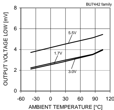
Fig.123 Output Voltage Low – Ambient Temperature (RL=10[kΩ])
