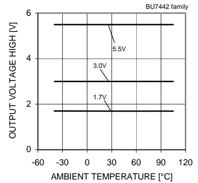
Fig.121 Output Voltage High – Ambient Temperature (RL=10[kΩ])
