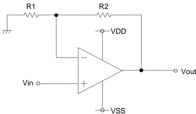
Fig.192 Non-inverting amplifier
