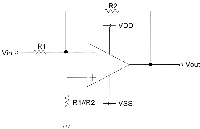
Fig.191 Inverting amplifier
