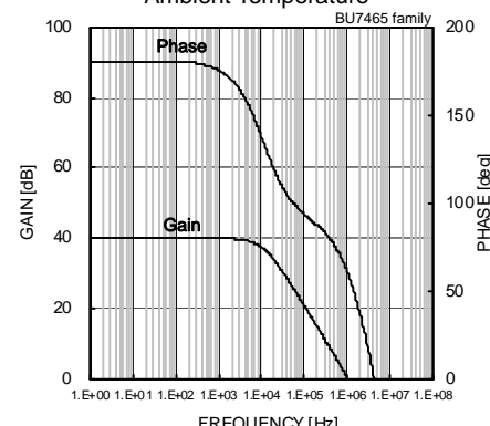
Fig.92 Gain – Frequency
