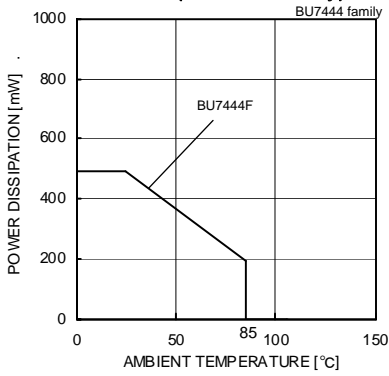
Fig.139 Derating curve
