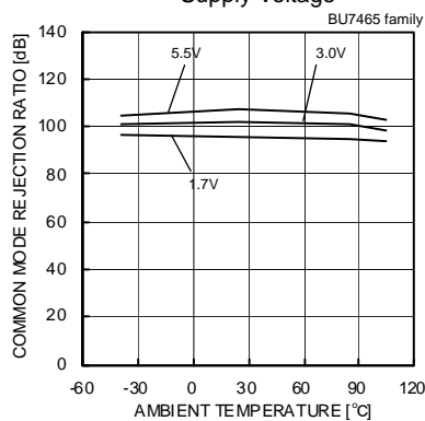
Fig.88 Common Mode Rejection Ratio – Ambient Temperature
