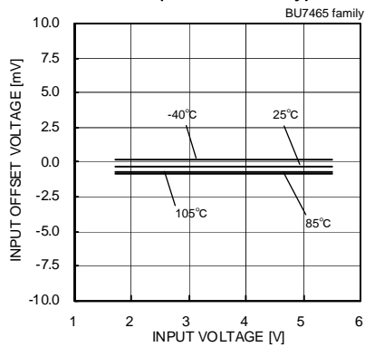
Fig.82 Input Offset Voltage – Supply Voltage (Vicm= VDD-1.2[V], VOVT= VDD/2)
