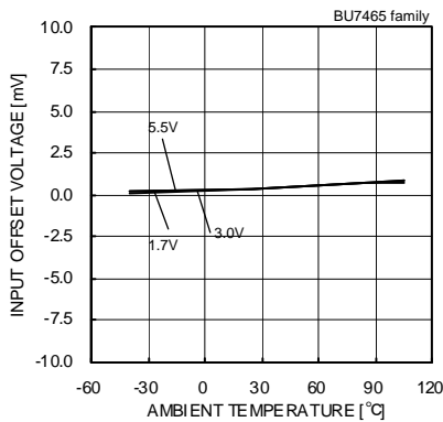
Fig.83 Input Offset Voltage – Ambient Temperature (Vicm= VDD-1.2[V], VOVT= VDD/2)
