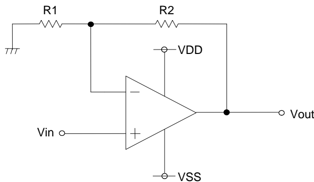
Fig.192 Non-inverting amplifier
