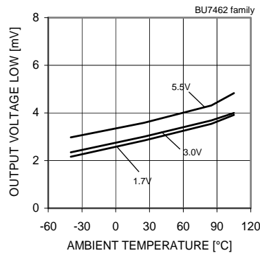
Fig.31 Output Voltage Low – Ambient Temperature (RL=10[kΩ])
