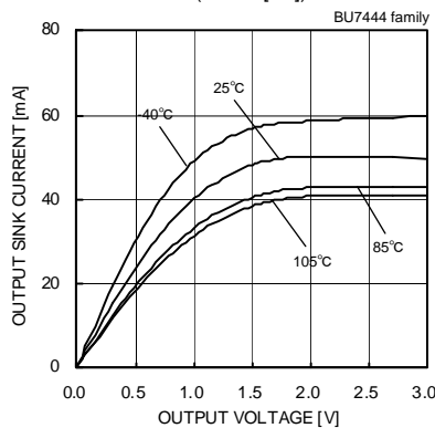
Fig.149 Output Sink Current – Output Voltage (VDD=3[V])
