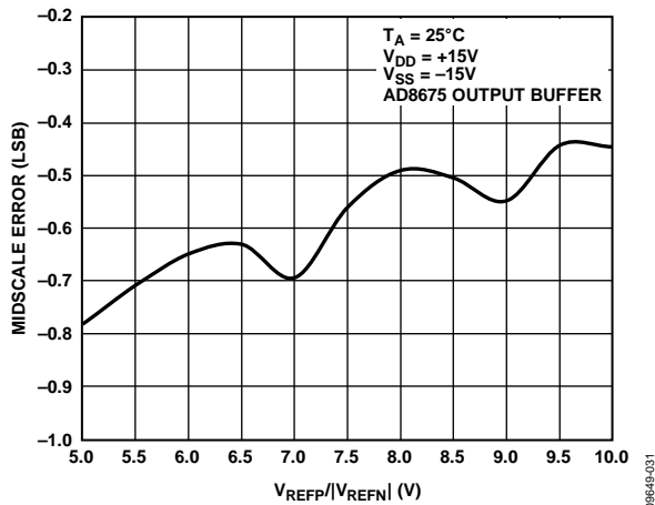
Figure 31. Midscale Error vs. Reference Voltage
