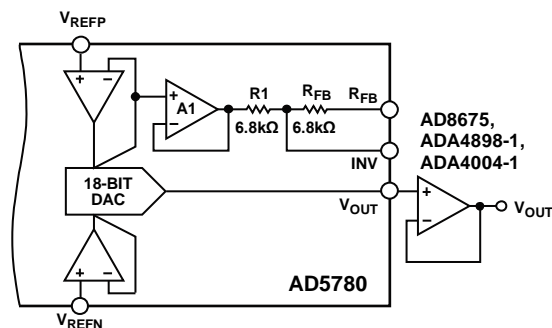
Figure 52. Output Amplifier in Unity-Gain Configuration
