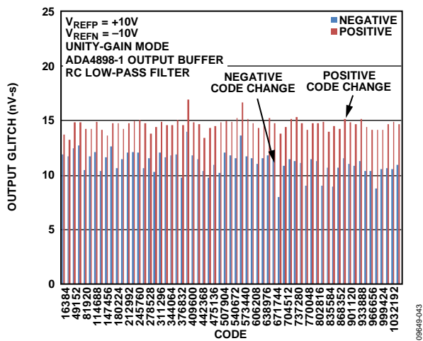
Figure 43. 6 MSB Segment Glitch Energy for \pm 10V_{REF}
