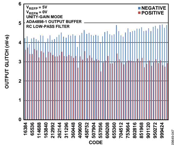
Figure 45. 6 MSB Segment Glitch Energy for 5V_{REF}
