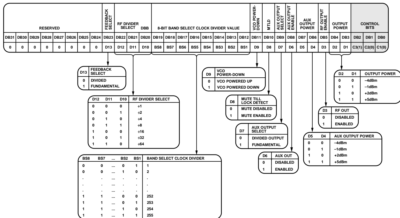
Figure 28. Register 4 (R4)
