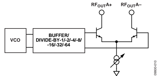
Figure 22. Output Stage
