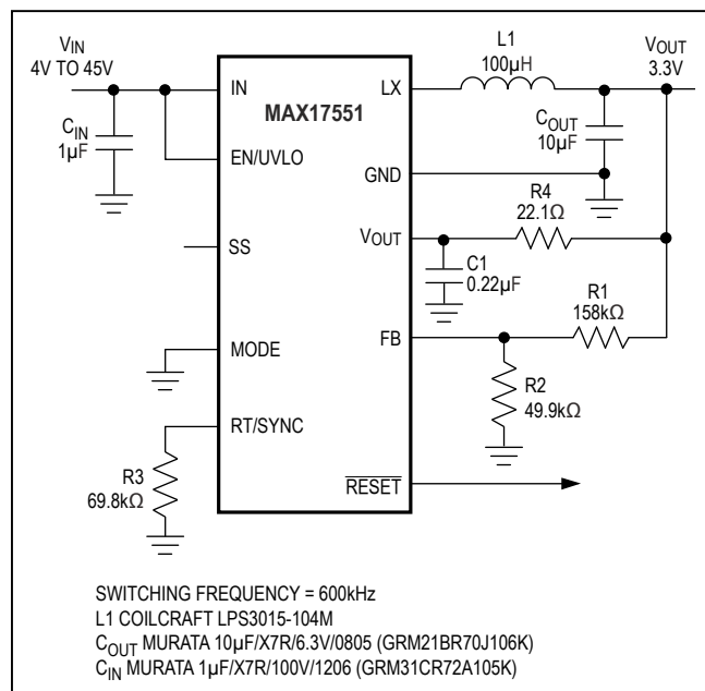
Figure 9. Small-Footprint 3.3V, 50mA Regulator
