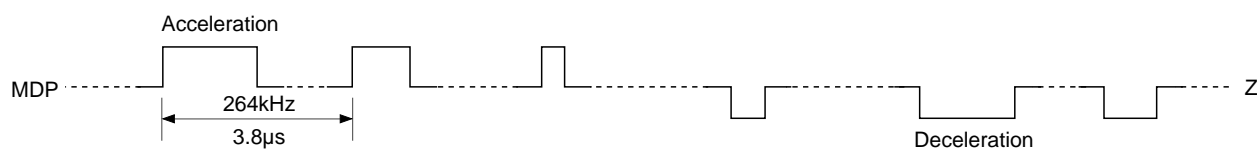
Timing Chart 2-13
