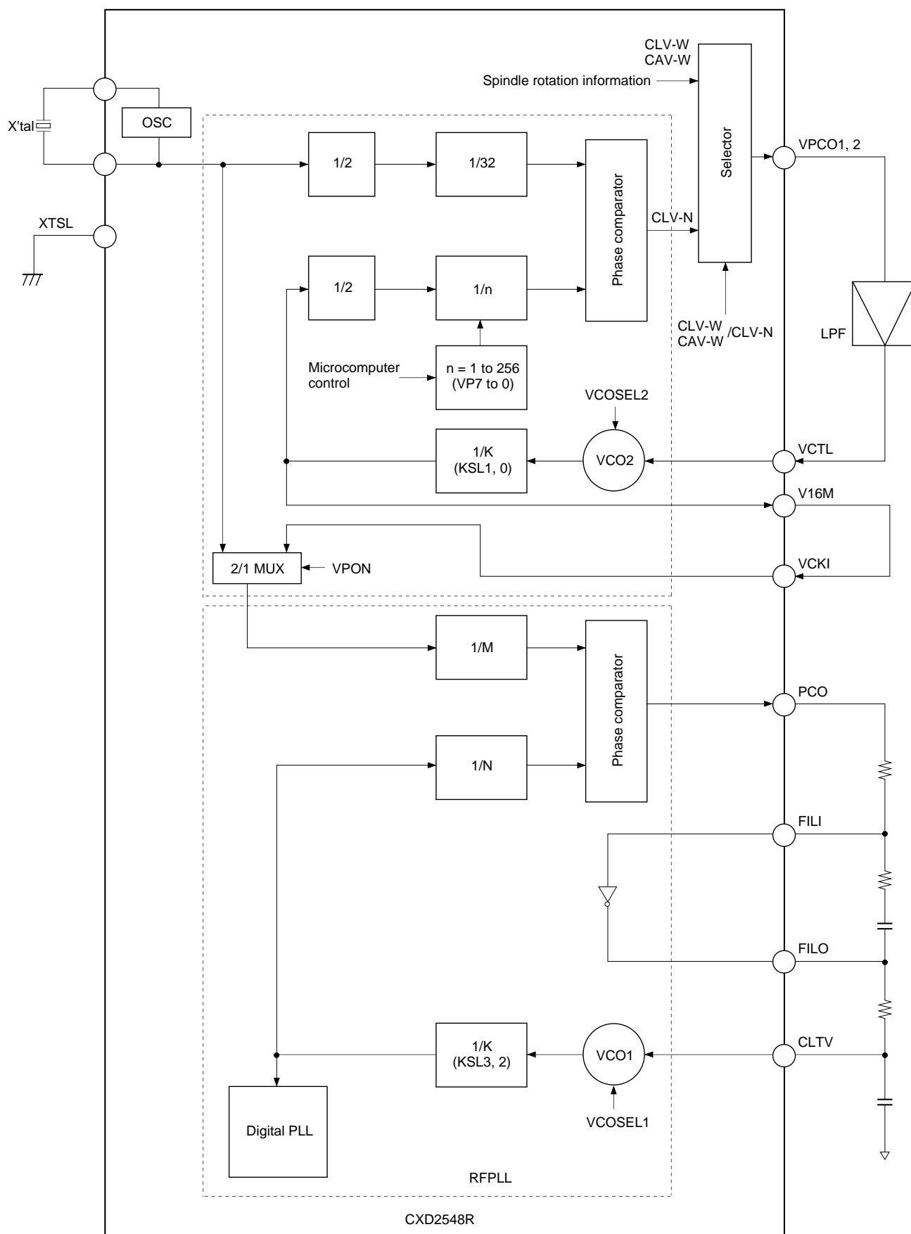
Block Diagram 3-10
