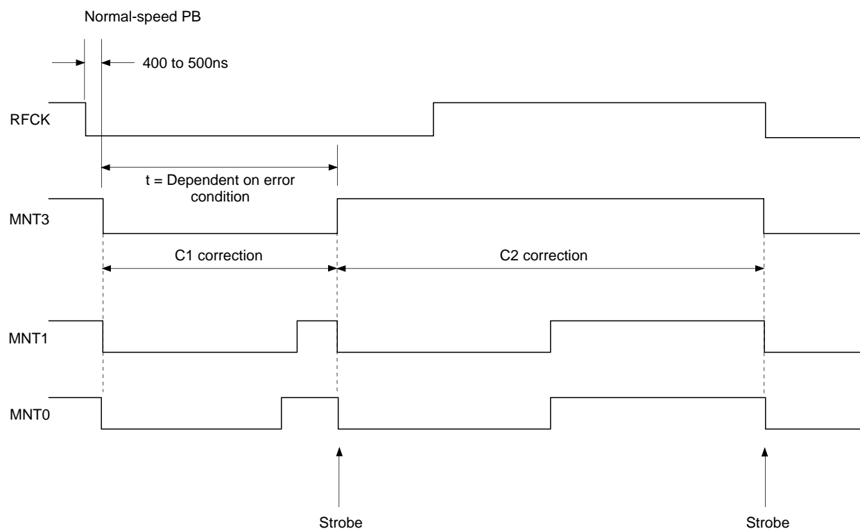
Timing Chart 3-1
