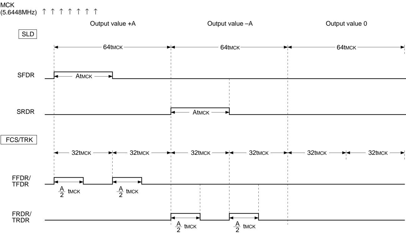
Timing Chart 4-3.
