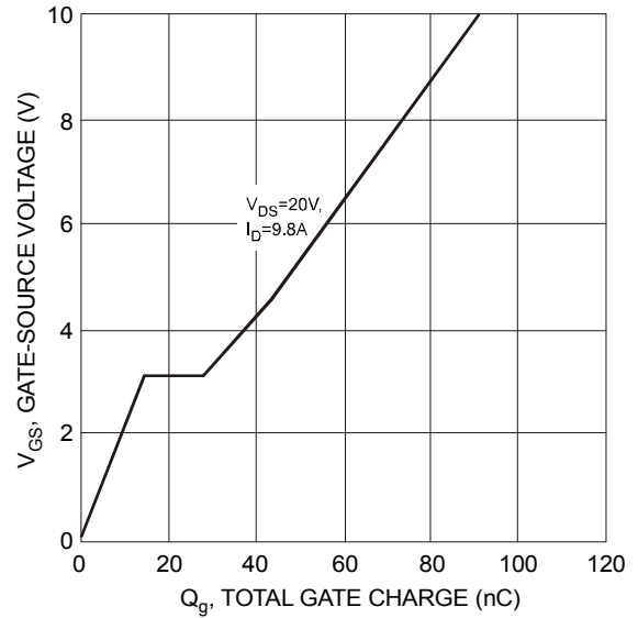
Fig. 10 Gate-Charge Characteristics
