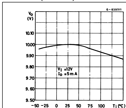
Figure 10. Output voltage vs. temperature (L4940V10)
