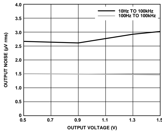
Figure 27. Output Noise vs. Output Voltage ( V_{OUT} )
