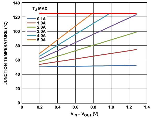
Figure 55. 100 mm 2 of PCB Copper, T_B = 50^\circ\text{C}
