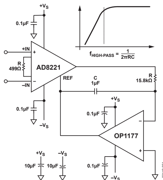
Figure 52. AC-Coupled Circuit
