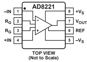
Figure 3. Pin Configuration
