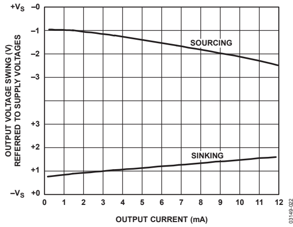
Figure 23. Output Voltage Swing vs. Output Current, G = 1
