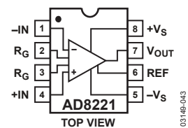
Figure 44. Pinout Diagram
