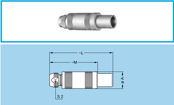
FFF Straight plug, non-latching, cable collet
