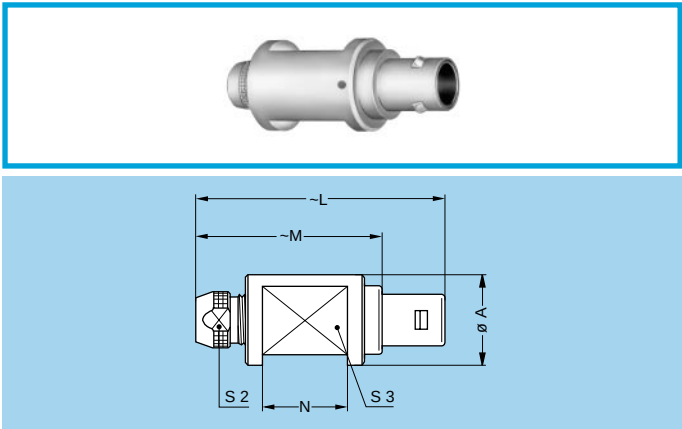
FZP Straight plug for remote handling, cable collet and inner anti-rotating device
