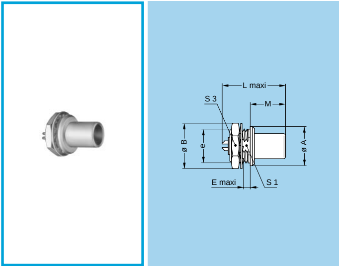
FAA Fixed plug non-latching, nut fixing
