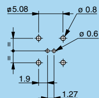
P19 - EPG-EXG (0B/1B.302) Screw mount
