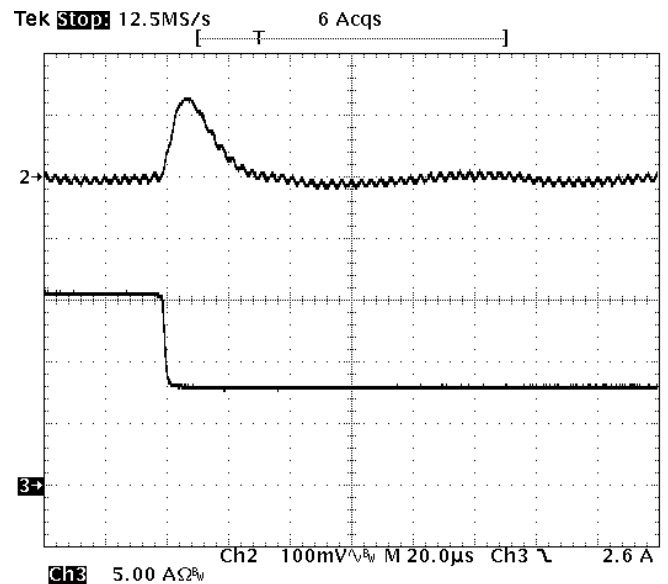
Fig-1.8V-7: Output voltage response for V_{out}=1.8V to negative load current step change from 16A to 8A with slew rate of -5A/us at V_{in}=12V . C_o=47uF \times 4 ceramic. Top trace: output voltage (100mV/div.) Bottom trace: load current (5A/div.) Time scale: 20us/div.
