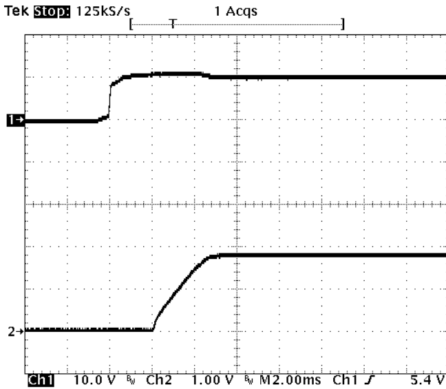
Fig-1.8V-4: Turn-on transient for V_{out}=1.8V with application of V_{in} at full rated load current (resistive) and 47uF \times 4 external capacitance at V_{in}=12V . Top trace: V_{in} (10V/div.) Bottom trace: output voltage (1V/div.) Time scale: 2 ms/div.
