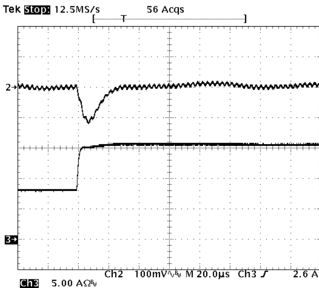
Fig-1.8V-6: Output voltage response for V_{out}=1.8V to positive load current step change from 8A to 16A with slew rate of 5A/us at V_{in}=12V . C_o=47uF \times 4 ceramic. Top trace: output voltage (100mV/div.) Bottom trace: load current (5A/div.) Time scale: 20us/div.
