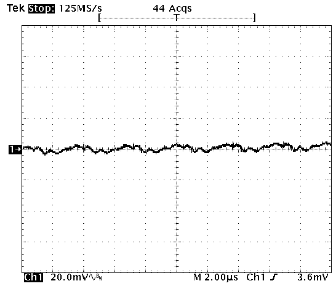
Fig-1.8V-5: Output voltage ripple (20mV/div.) for V_{out}=1.8V at full rated load current into a resistive load with external capacitance 47uF \times 4 ceramic + 1uF ceramic at V_{in}=12V . Time scale: 2 us/div
