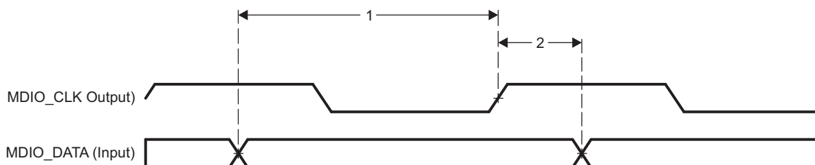
Figure 5-2. MDIO_DATA Timing - Input Mode
