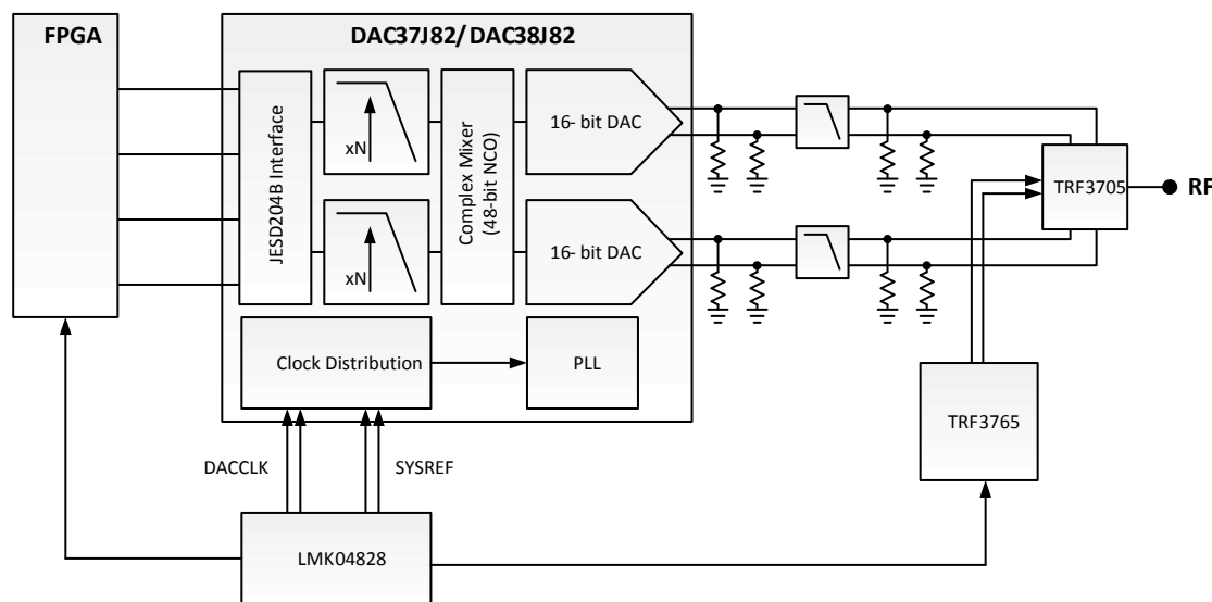
Figure 81. Low-IF Wideband LTE Transmitter Diagram
