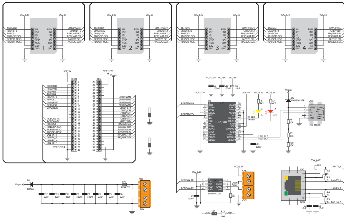
Figure 19-2: mikromedia+ SHIELD for PIC32MX7® schematic
