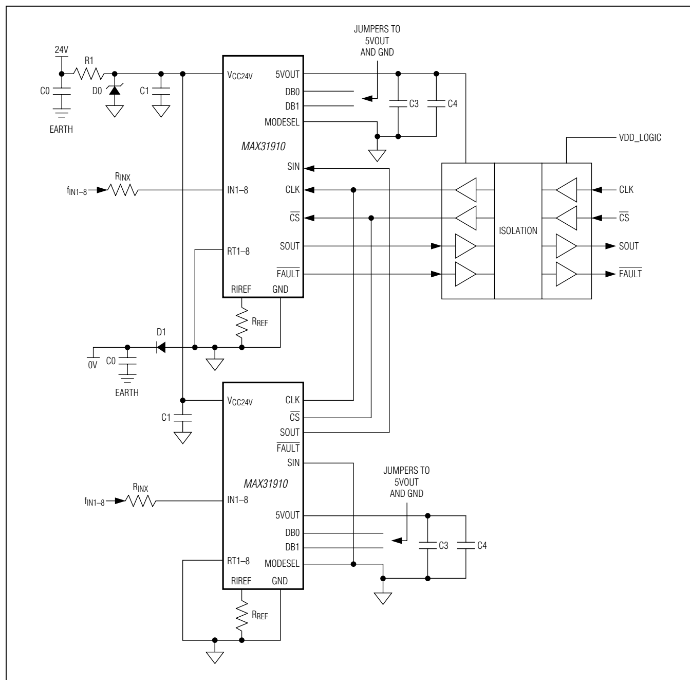
Figure 5. 16-Input Application Circuit
