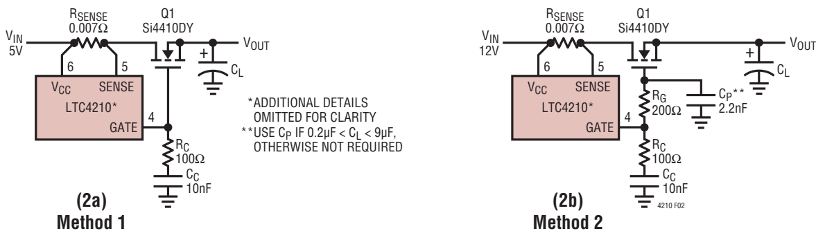
Figure 2. Frequency Compensation
