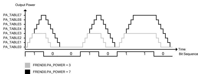
Figure 56: PA_POWER and PA_TABLE
