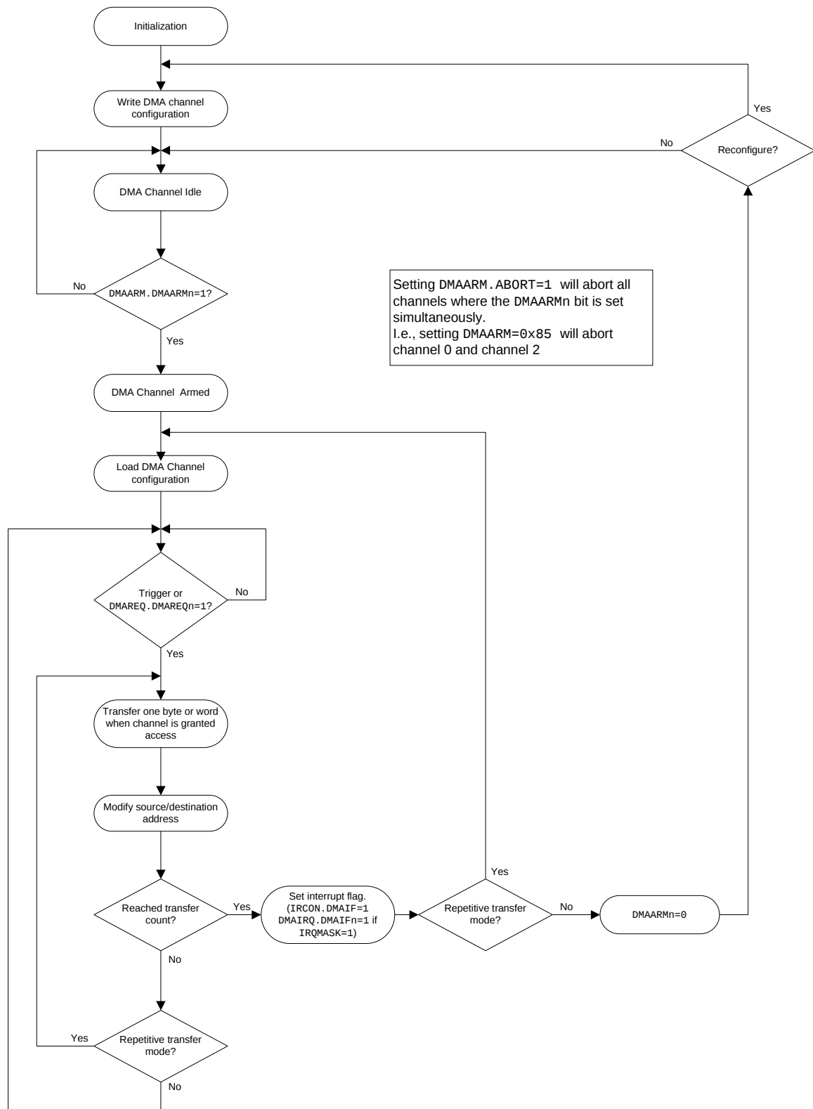
Figure 26: DMA Operation
