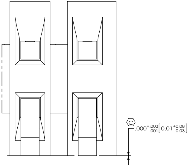
DETAIL 'C' SCALE 20 : 1
