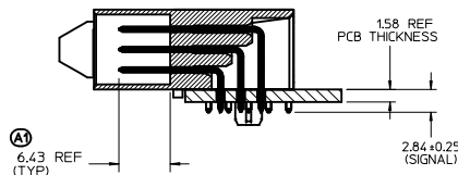
SECTION Z-Z
