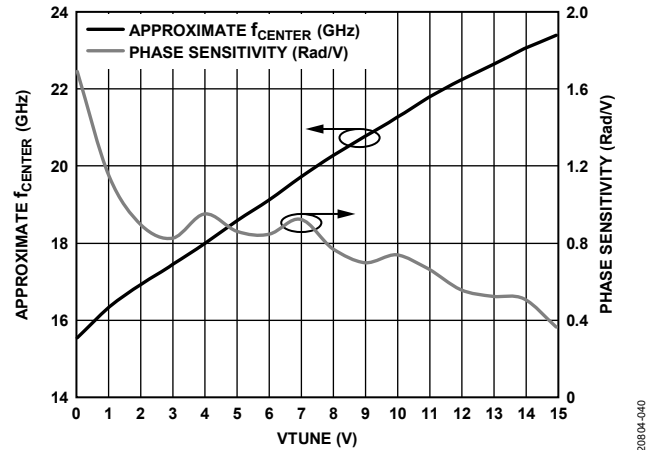
Figure 40. Approximate f_{\text{CENTER}} and Phase Sensitivity vs. VTUNE
