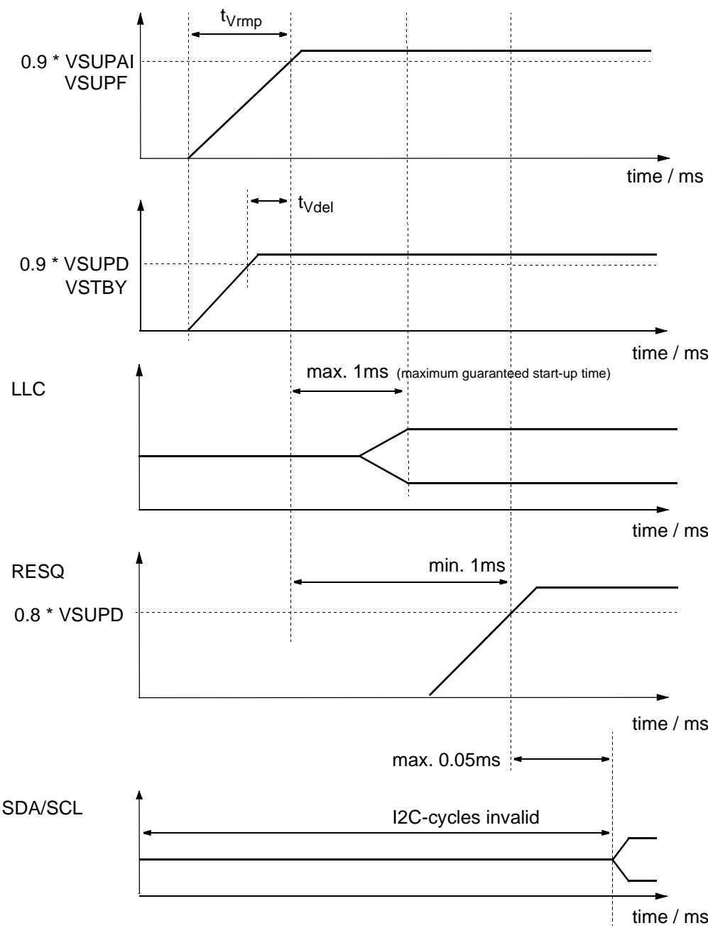
Fig. 4–13: Power-Up sequence
