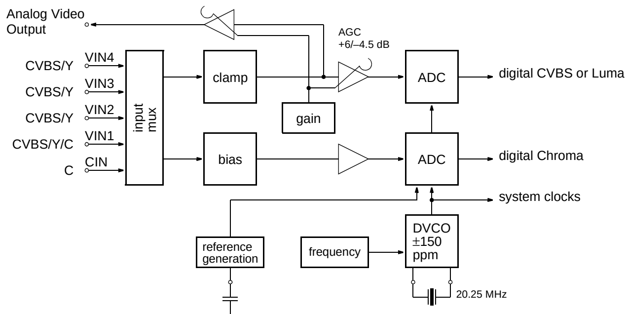
Fig. 2–1: Analog front-end
