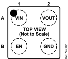
Figure 4. Pin Configuration
