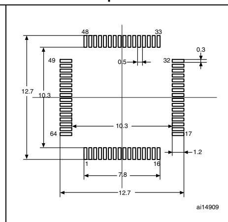
Figure 59. Recommended footprint (1)(2)
