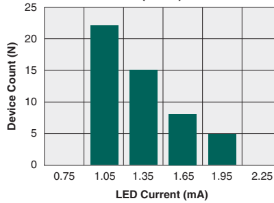
Typical I F for Switch Dropout (N=50)
