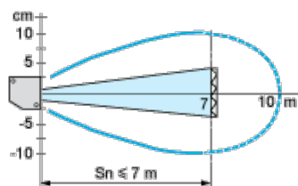
With reflector XU5C50
