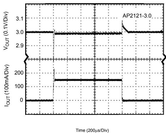
Figure 22. Load Transient (Conditions: V_{IN}=4\text{V} , C_{IN}=1\mu\text{F} , C_{OUT}=1\mu\text{F} )
