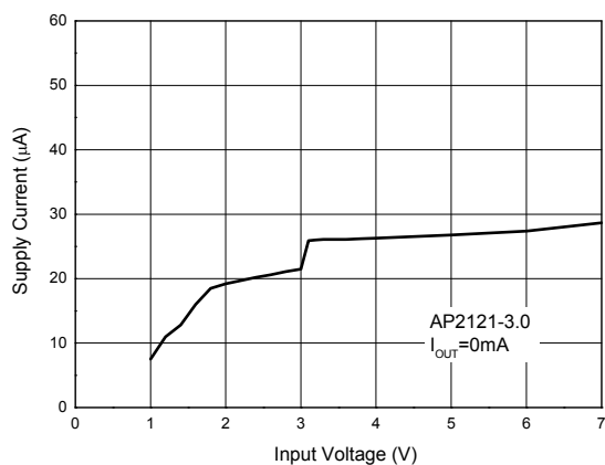
Figure 16. Supply Current vs. Input Voltage
