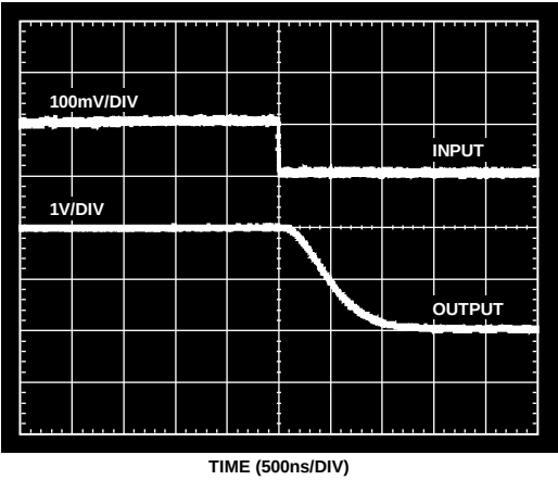
Figure 13. Fall Time
