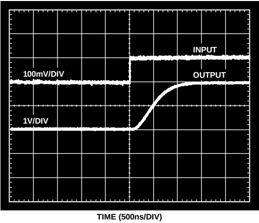
Figure 14. Rise Time
