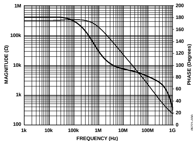
Figure 37. Transimpedance
