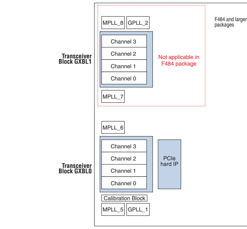
Figure 1–2. F484 and Larger Packages with Transceiver Channels for Cyclone IV GX Devices
