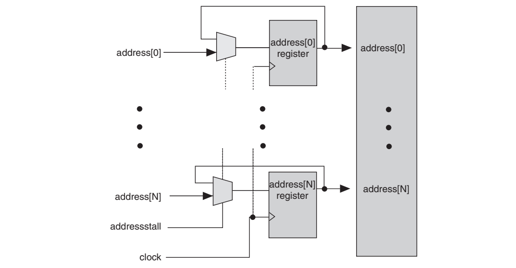
Figure 3–2. Cyclone IV Devices Address Clock Enable Block Diagram
