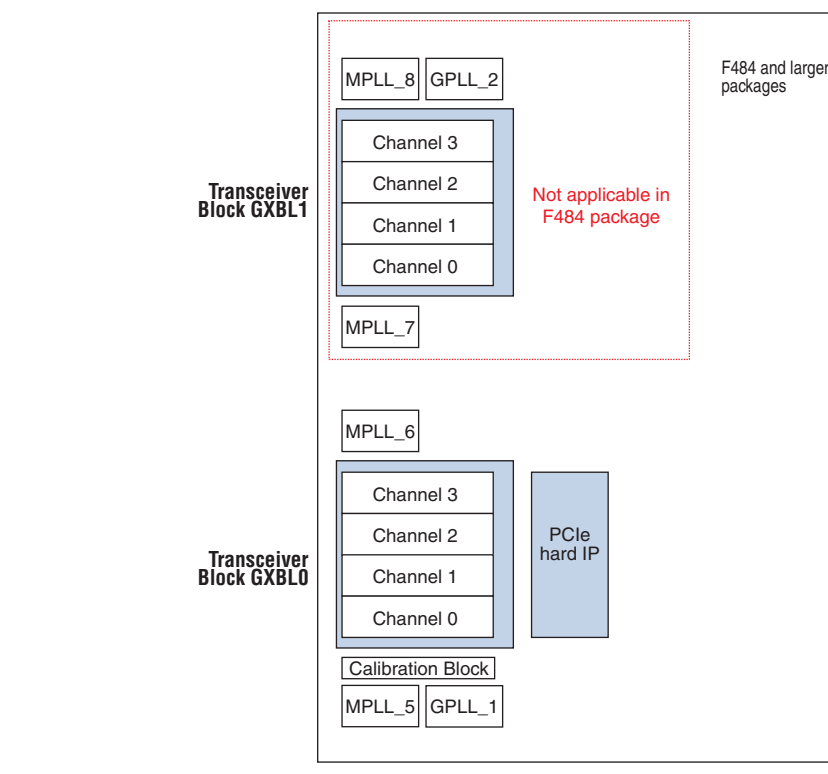
Figure 1–2. F484 and Larger Packages with Transceiver Channels for Cyclone IV GX Devices
