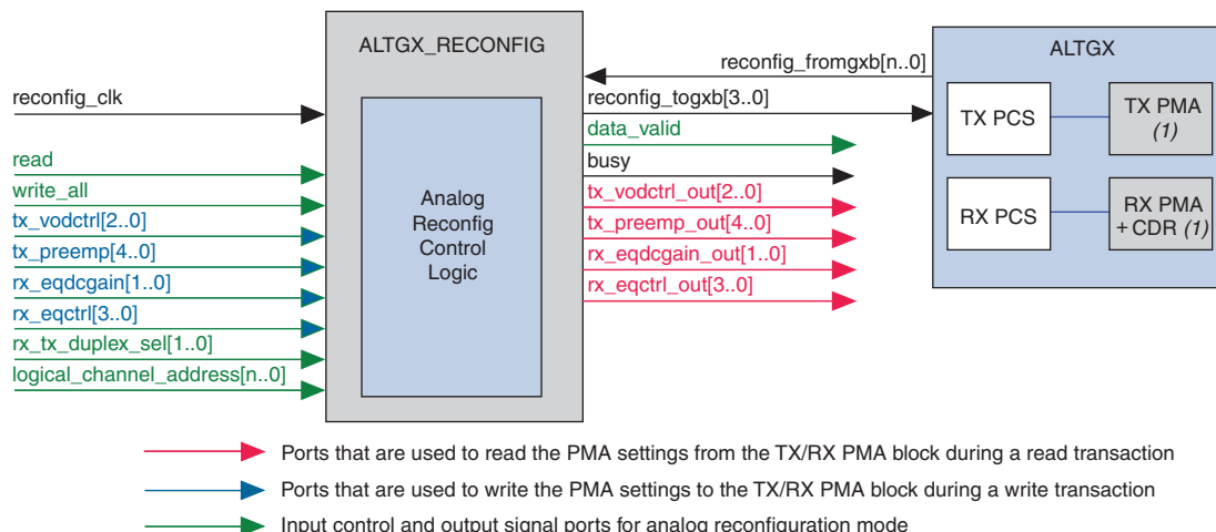
Figure 3–9. ALTGX and ALTGX_RECONFIG Connection for PMA Reconfiguration Mode
