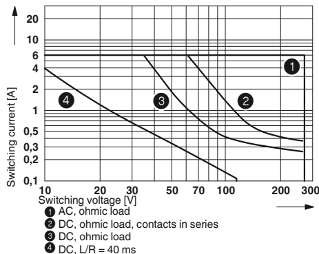
Electrical interrupting rating for PLC...11C/ACT for high inrush currents
