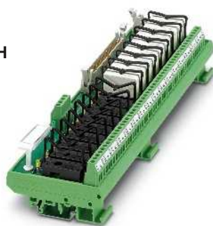
Output base module with 16 miniature relays, 1 PDT
