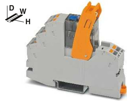
RIF-1 relay module with 1 PDT relay with manual operation
