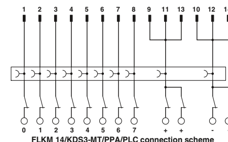
FLKM 14/KDS3-MT/PPA/PLC connection scheme
