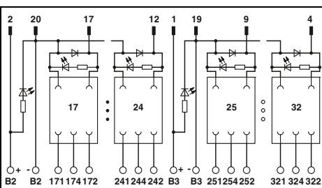
Output extension module with 16 miniature relays, 1 PDT
