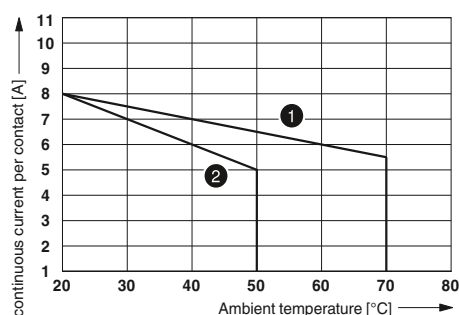
Contact derating
