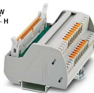
VARIOFACE termination board for 16 channels with push-in connection
