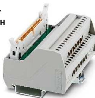
VARIOFACE termination board for 16 channels with screw connection
