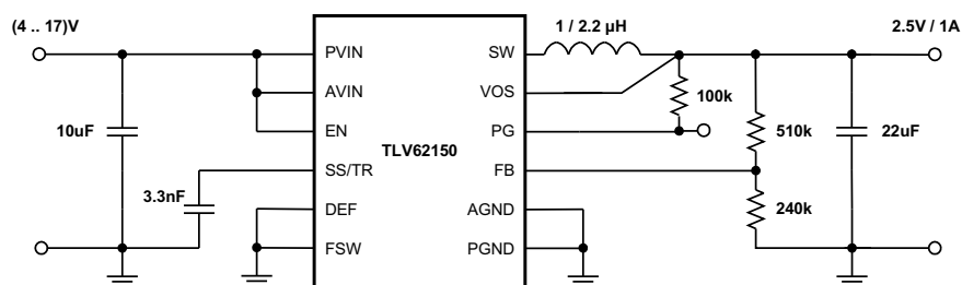
Figure 41. 2.5-V/1-A Power Supply
